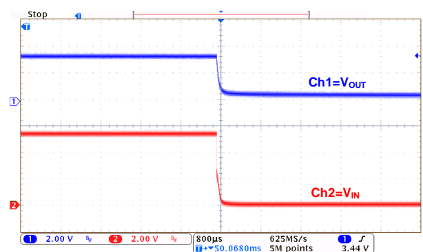
Power-Down: HL8333 ( I_{OUT}=0mA )
