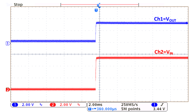
Power-Up: HL8333 ( I_{OUT}=0mA )
