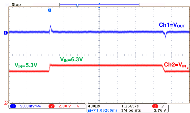
Line Transient: HL8333 ( I_{OUT}=1mA )
