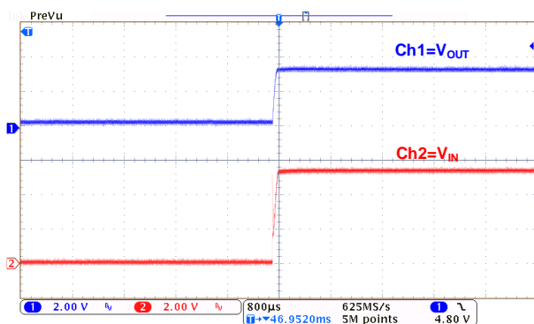
Power-Up: HL8333 ( I_{OUT}=300mA )
