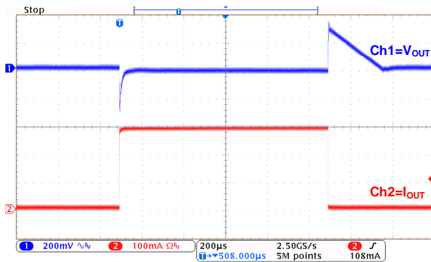
Load Transient: HL8333 ( I_{OUT}=1mA\sim 300mA\sim 1mA )
