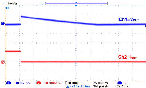
Load Transient: HL8333( I_{OUT}=50mA\sim 0mA )
