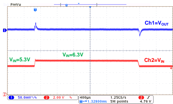
Line Transient: HL8333 ( I_{OUT}=10mA )
