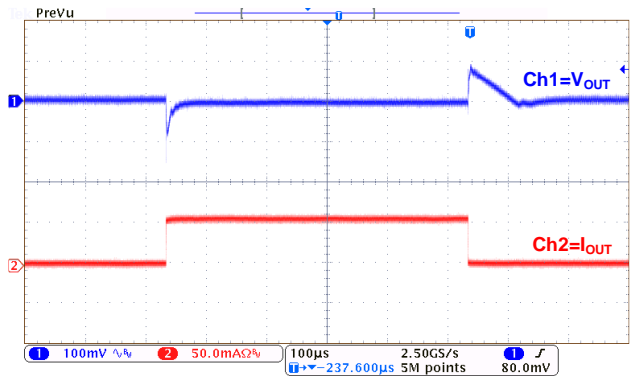
Load Transient: HL8333( I_{OUT}=1mA\sim 50mA\sim 1mA )
