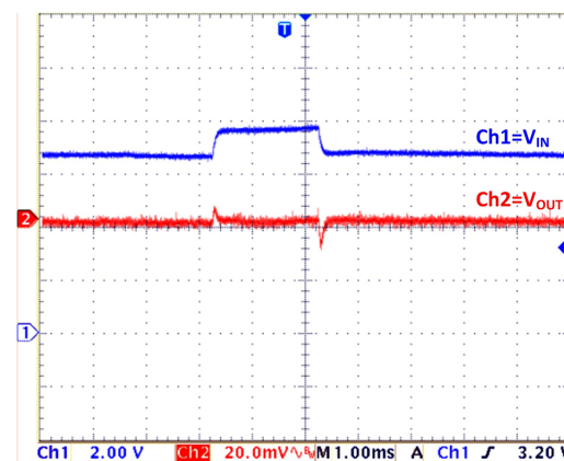
Line Transient:
