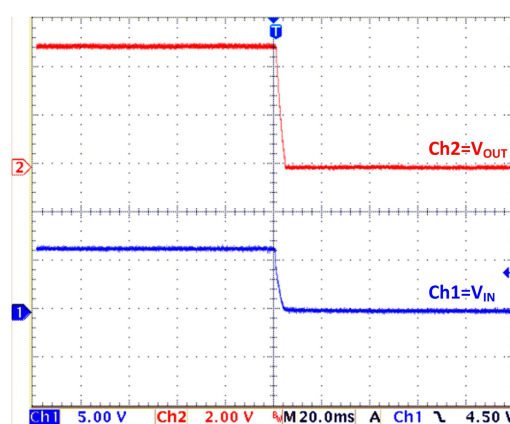
Power-Down:
