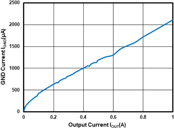
GND Current vs Output Current at V_{OUT}=5.0V
