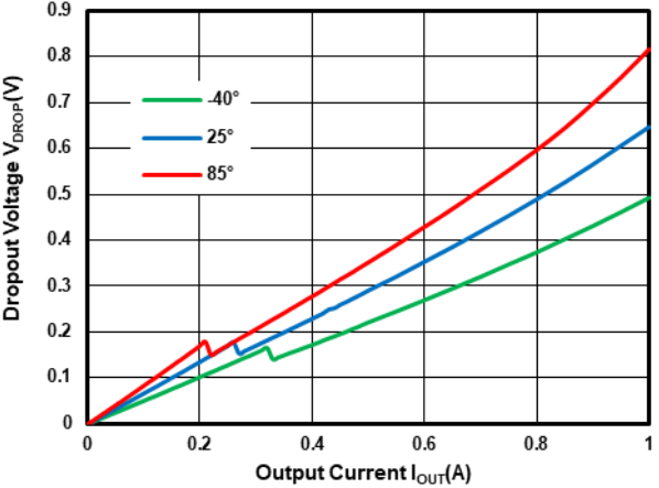
Dropout Voltage vs Temperature at V_{OUT}=5.0V
