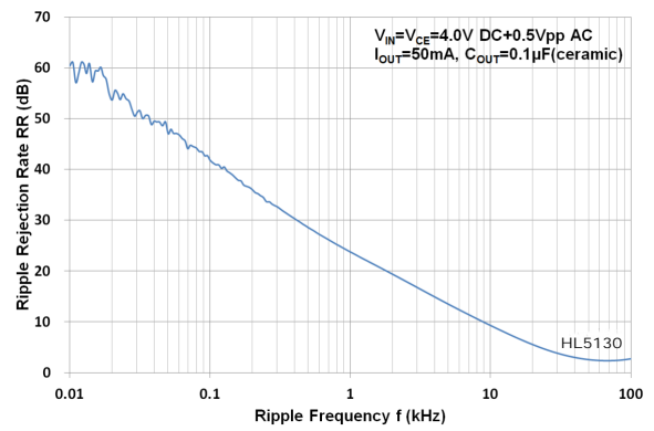
HL5130 Power Supply Rejection Ratio
