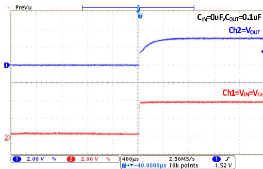
Power Up: HL5130 ( I_{OUT}=1mA )
