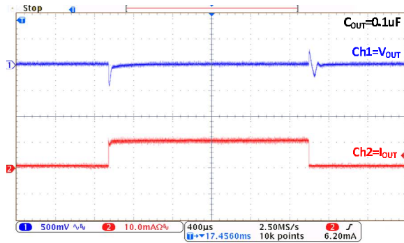
Load Transient: HL5130 ( I_{OUT}=1mA\sim 10mA\sim 1mA )
