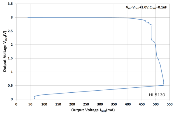
HL5130 Output Current Fold-back
