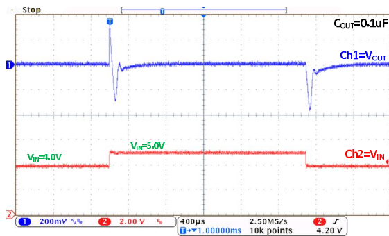
Line Transient: HL5130 ( I_{OUT}=1mA )
