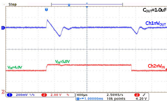
Line Transient: HL5130 ( I_{OUT}=1mA )
