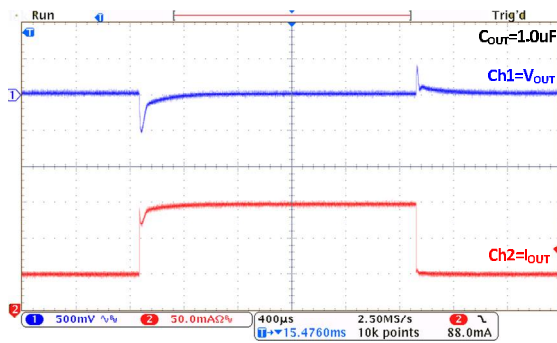
Load Transient: HL5130 ( I_{OUT}=50mA\sim 100mA\sim 50mA )
