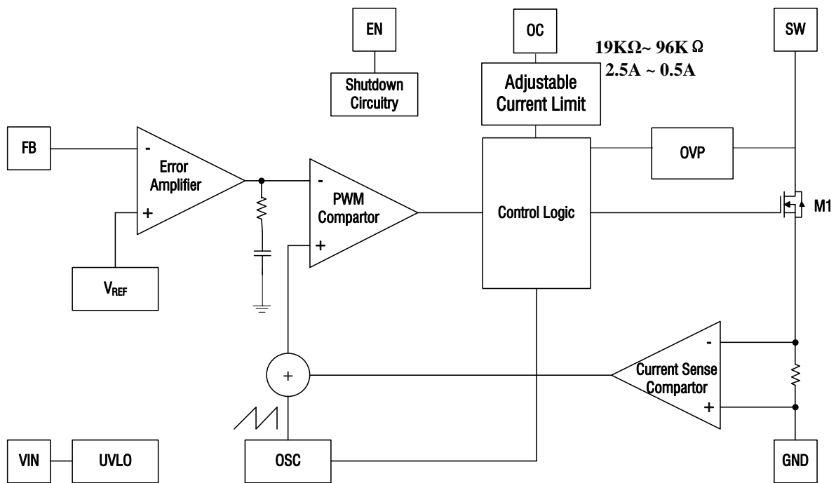
Figure 2. HL9710L Block Diagram
