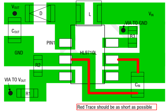
Figure 3. HL9710L Suggested Layout
