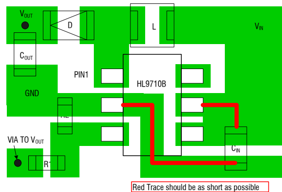
Figure 3. HL9710B Suggested Layout
