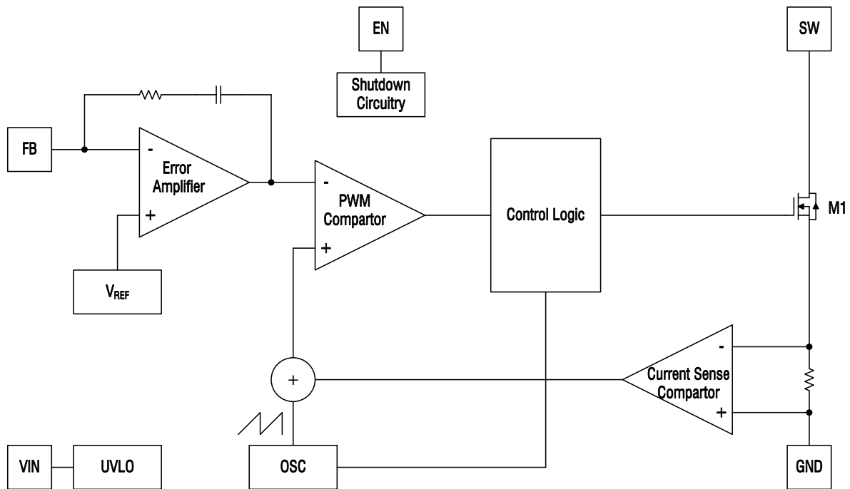
Figure 2. HL9710B Block Diagram
