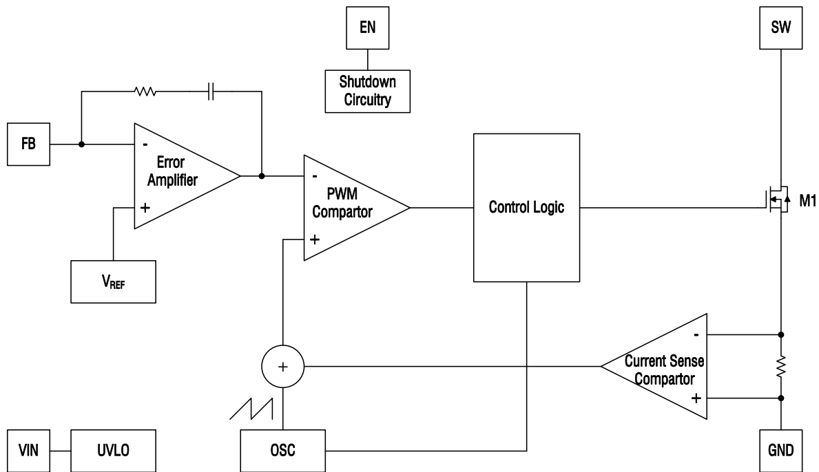
Figure 2. HL9710 Block Diagram
