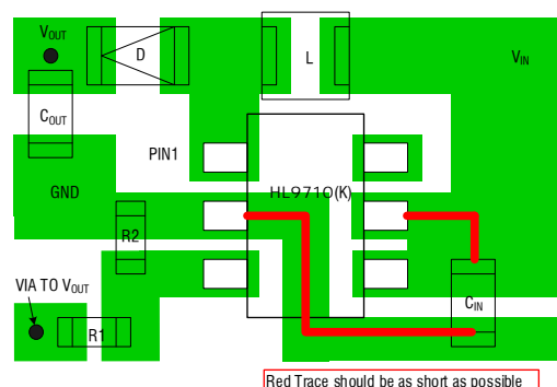
Figure 3. HL9710 Suggested Layout
