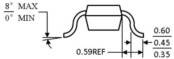
Figure 23 6-Lead Small Outline Transistor Package [SOT-23]
