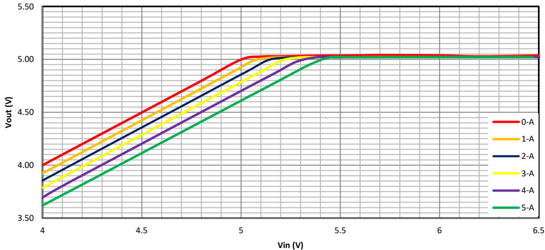
Figure 11. LDO Operation Characteristic ( Vout =5V )
