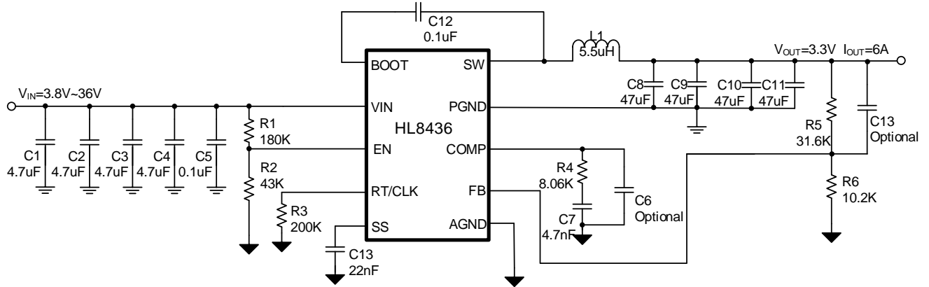
Figure 12. HL8436 Design Example, 3.3V Output with Programmable UVLO
