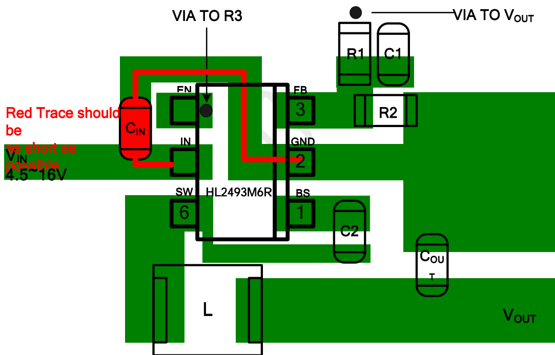
Figure 3. HL2493M6R Suggested Layout
